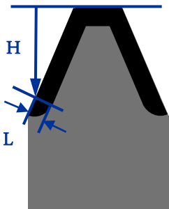
Carburized Induction Hardening
