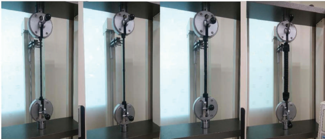
FIG 3. PULLING OUT TEST (07,10,12,22)
